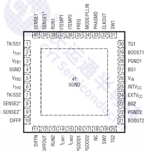
QFN40 (6mm×6mm)
